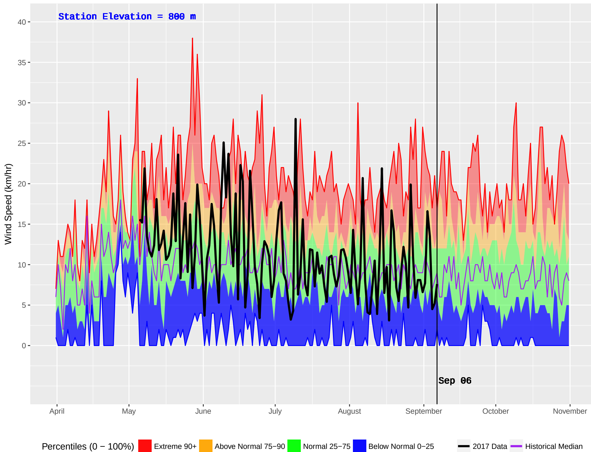
DEASE LAKE FS (108) : Historical (1978–2016) and Current (2017) Noon Wind Speed
