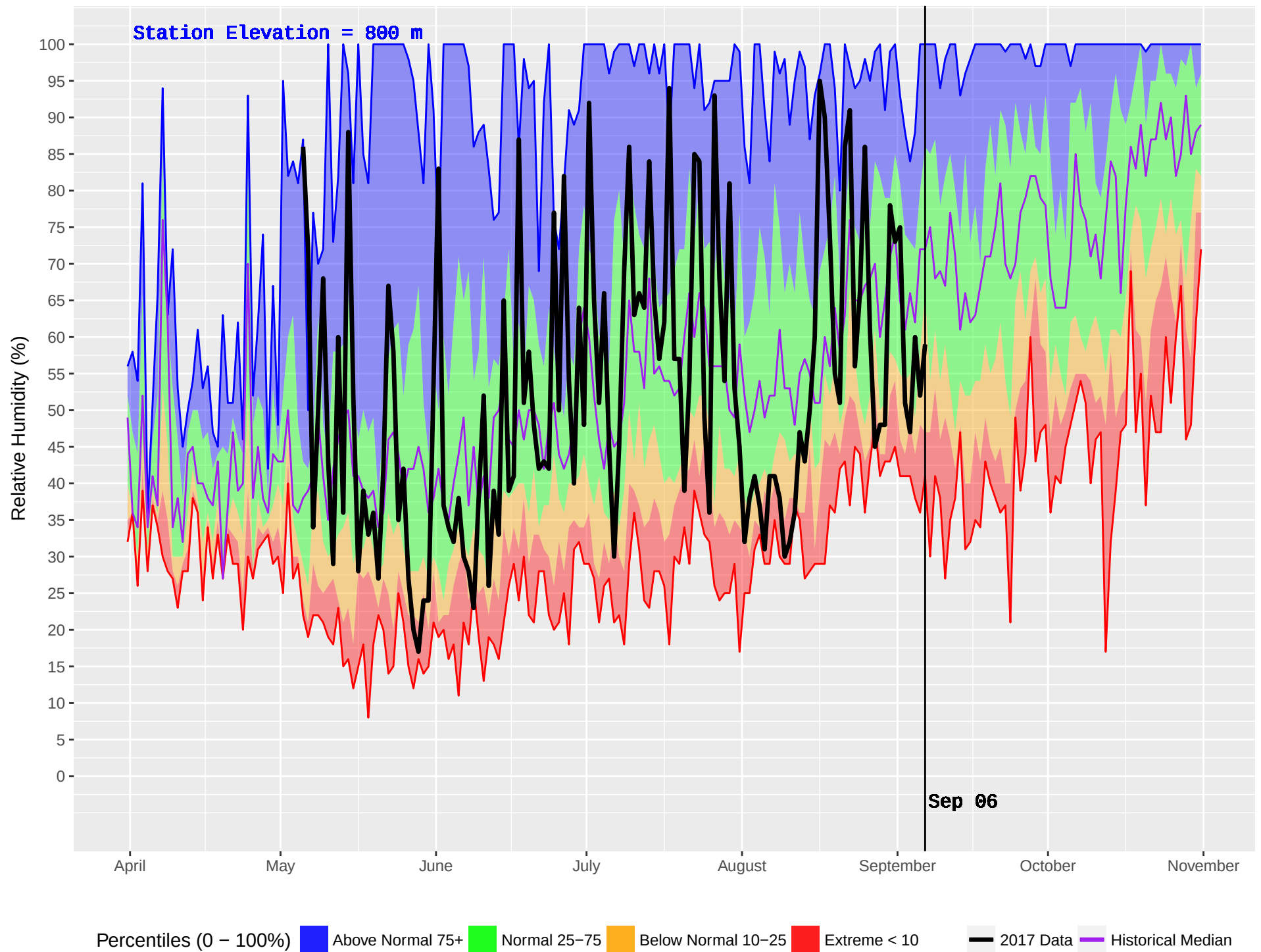
DEASE LAKE FS (108) : Historical (1978–2016) and Current (2017) Noon Relative Humidity
