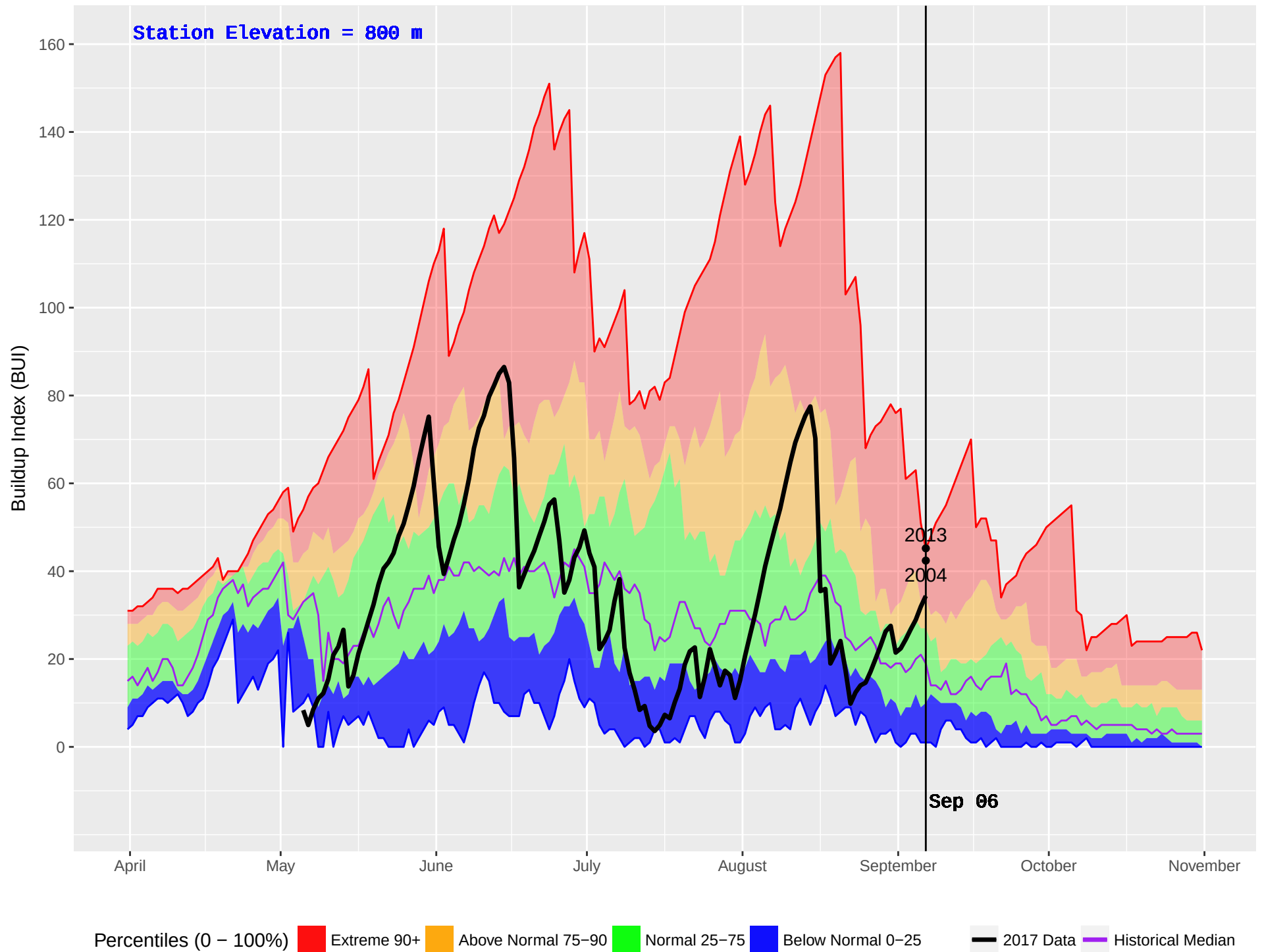
DEASE LAKE FS (108) : Historical (1978–2016) and Current (2017) Noon Buildup Index (BUI)
